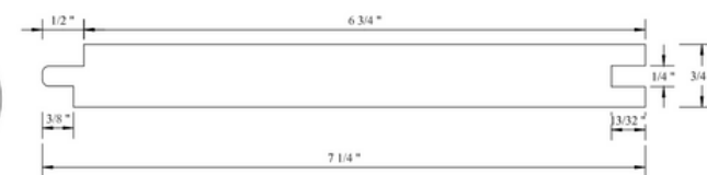
T & G #147C NICKLE GAP (1/8" Gap) 3/4" X 7 1/4" PINE T & G #147C NICKLE GAP (1/8" Gap) 3/4" X 7 1/4" WHITEWOOD
