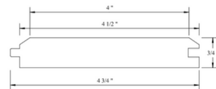
T & G 146A WHITEWOOD 3/4" x 4 3/4"
