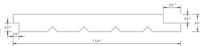
SHIPLAP #148C 1/2" GAP 3/4" X 7 1/4" PINE SHIPLAP #148C 1/2" GAP 3/4" X 7 1/4" WHITEWOOD
