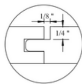
T & G #147B NICKLE GAP (1/8" Gap) 3/4" X 5 1/2" PINE T&G #147B NICKLE GAP (1/8" Gap) 3/4" X 5 1/2" WHITEWOOD
