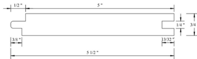
T & G #147B NICKLE GAP (1/8" Gap) 3/4" X 5 1/2" PINE T&G #147B NICKLE GAP (1/8" Gap) 3/4" X 5 1/2" WHITEWOOD
