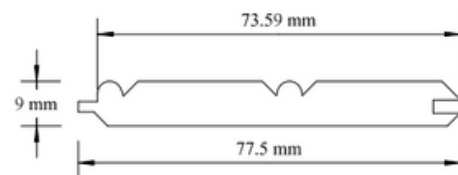
T & G 145 PINE 3/8" x 3 1/8" T & G 145 WHITEWOOD 3/8" x 3 1/8"
