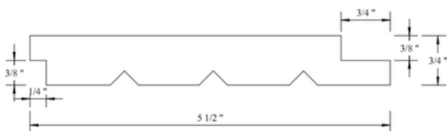
SHIPLAP #148B 1/2" GAP 3/4" X 5 1/2" PINE SHIPLAP #148B 1/2" GAP 3/4" X 5 1/2" WHITEWOOD
