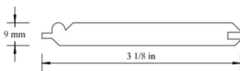
T & G 145S WHITEWOOD 3/8" x 3 1/8"
