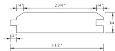
T & G 146 PINE 3/4" x 3 1/2"
